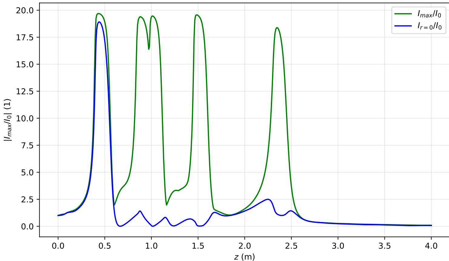
I_{max}(x = 0, y = 0, z)/I_0 , Pin=5.6Pcr, noisy input, artificial time
